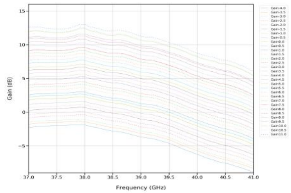
Figure 14. Rx Gain vs Frequency for RF 2
