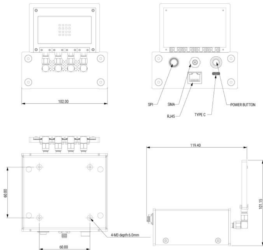
Figure 4. BBox™ Lite Dimension Drawing
