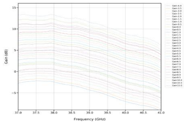
Figure 16. Rx Gain vs Frequency for RF 4
