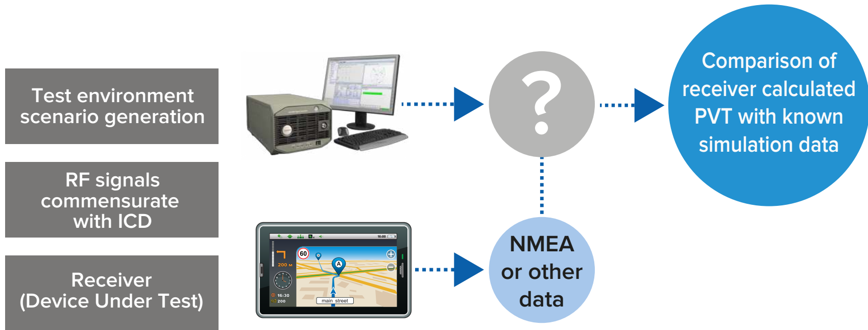
Figure 2. Simulation test set-up.
